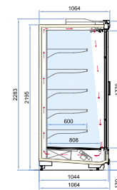
Palco D P105/H225 F30 L125-188-220-250-375
