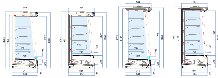
Palco P95/H205 F30 L125-188-250-375
