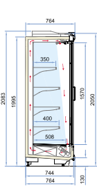
Palco D P75/H205 L125-146-188-250-375
