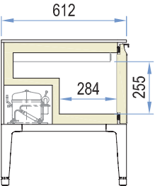
Neutral compartment with door Vano neutro con porta
