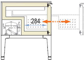
Neutral compartment with removable drawer Vano neutro con cassetto estraibile
