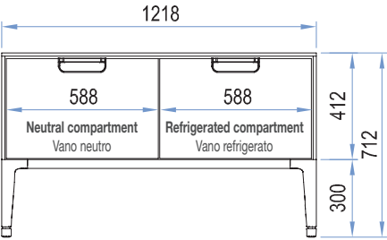
Removable drawers (2) Cassetti estraibili
