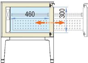
Refrigerated compartment with removable drawer Vano refrigerato con cassetto estraibile
